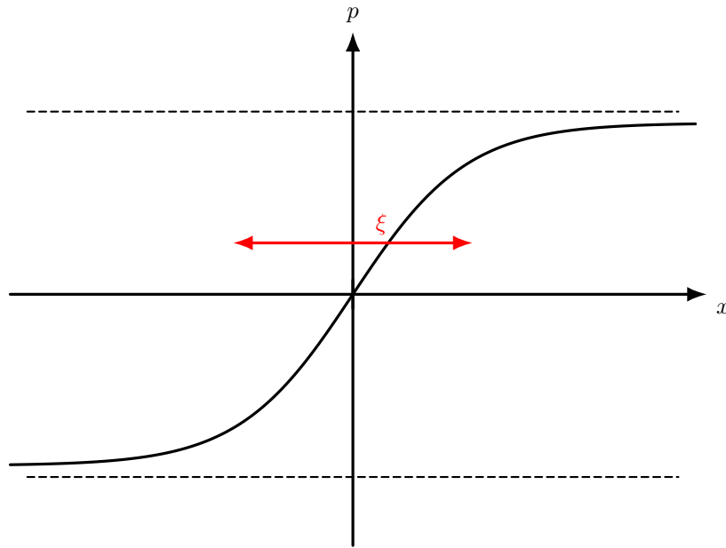
Figure 1.6: A smooth phase transition with Domain Wall \xi . (Converted from an iPad drawing using OpenAI Prism)
