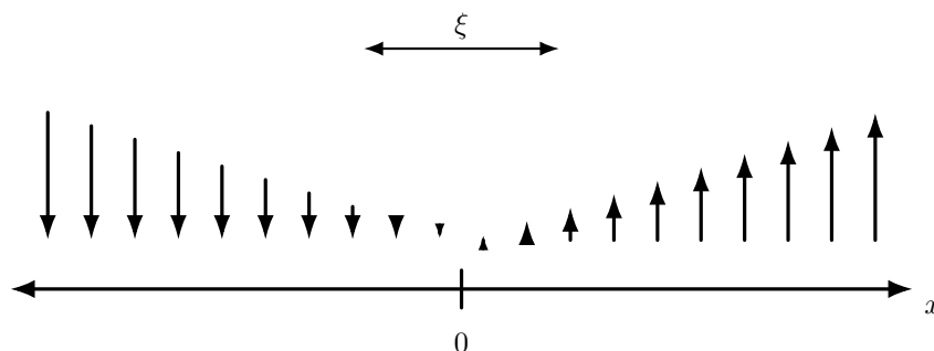
Figure 1.5: A smooth phase transition with Domain Wall \xi . (Converted from an iPad drawing using OpenAI Prism)
